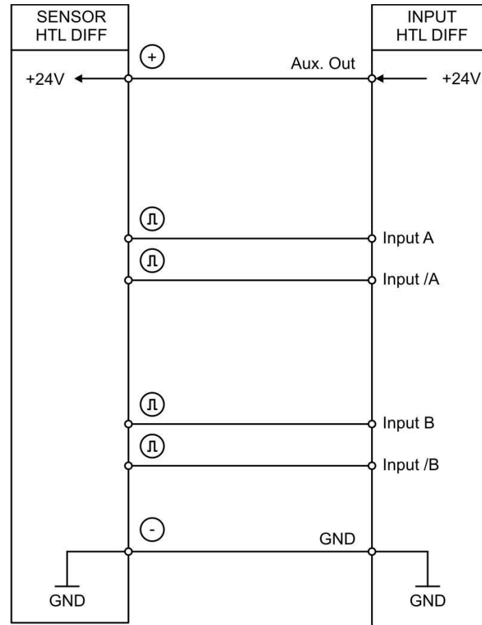
HTL DIFFERENTIAL
