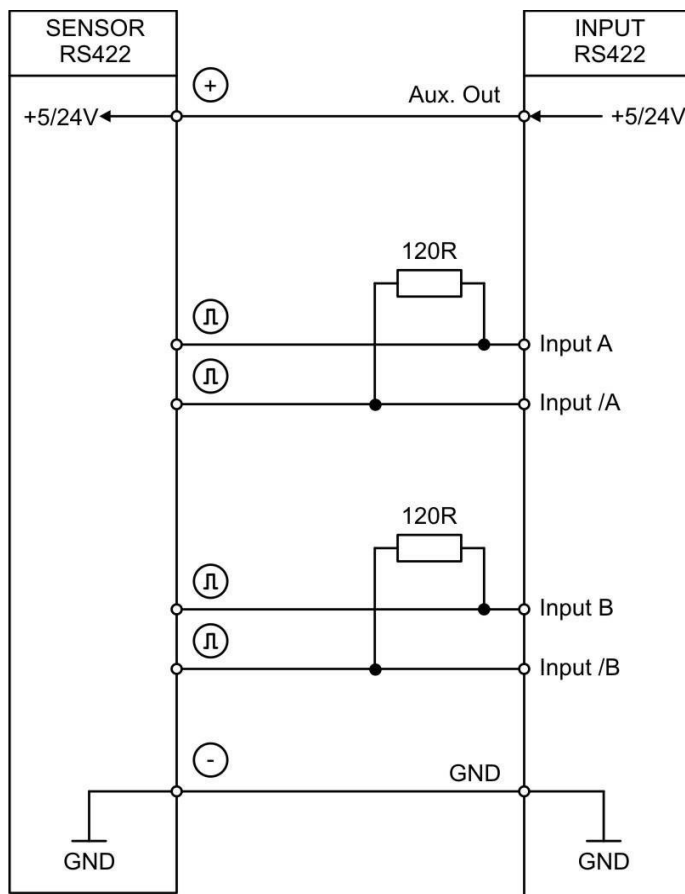
RS422
